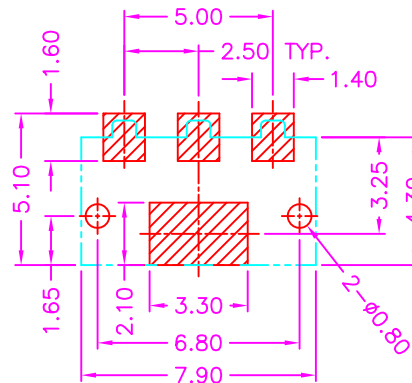
P.C.B. LAYOUT TOP VIEW ±0.05
