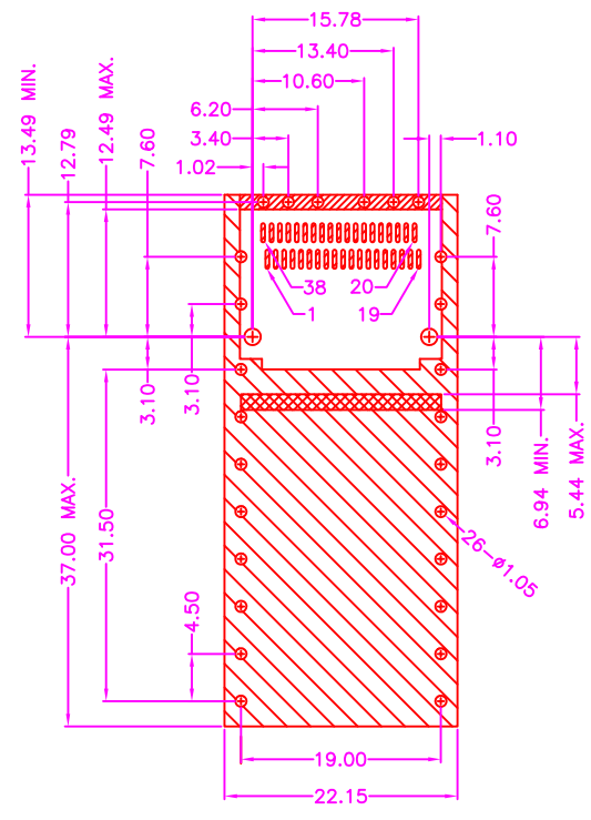
P.C.B LAYOUT TOP VIEW ±0.05
