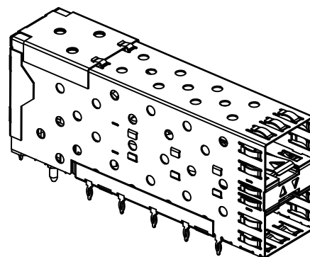
F21BD-0*C-131 WITH INNER LIGHT PIPES
