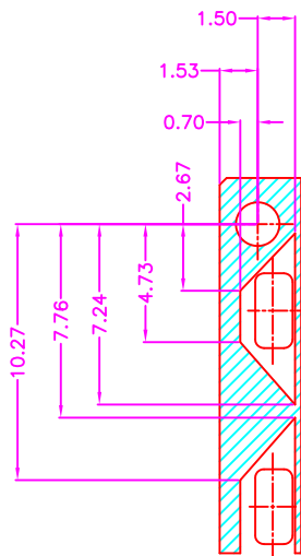
DETAIL C SCALE 2:1
