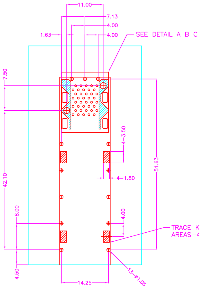
P.C.B. LAYOUT TOP VIEW ±0.05
