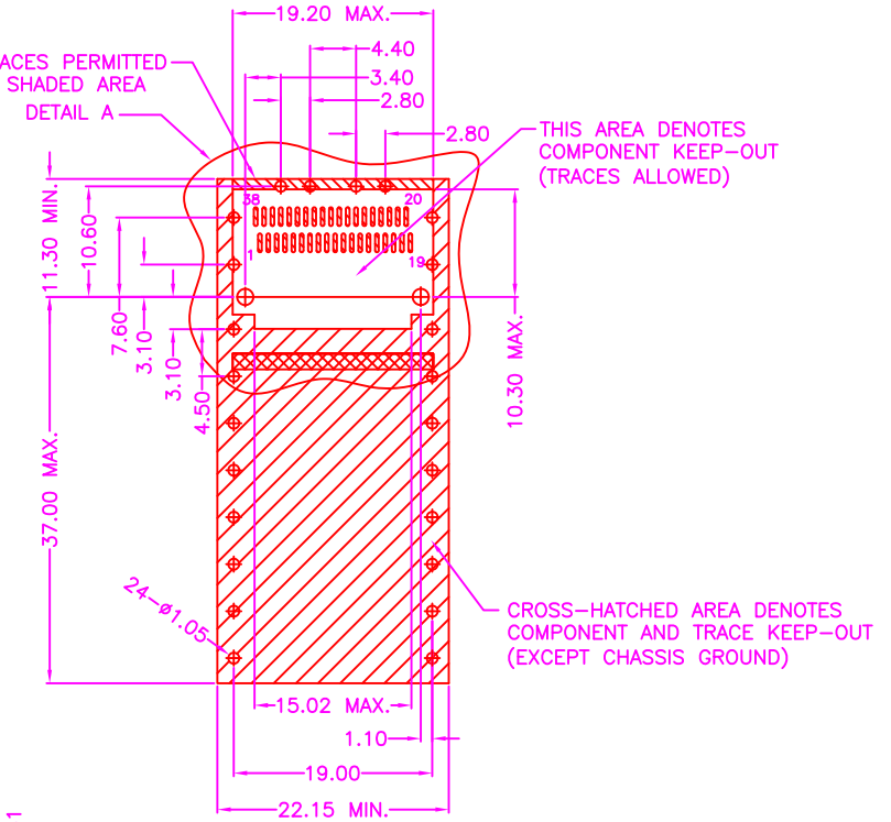
P.C.B. LAYOUT TOP VIEW ±0.05
