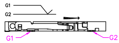
STEP III PUSH SHELL (G1/G2 SWITCH LOCK)
