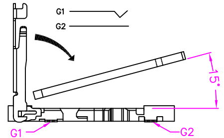
STEP I INSERT MICRO SIM CARD (G1/G2 SWITCH OPEN)
