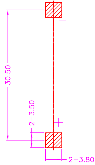
P.C.B. LAYOUT TOP VIEW ±0.05
