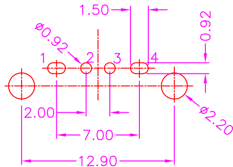
P.C.B. LAYOUT TOP VIEW ±0.05
