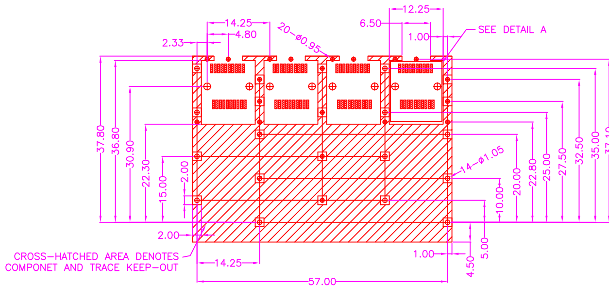
P.C.B LAYOUT TOP VIEW ±0.05
