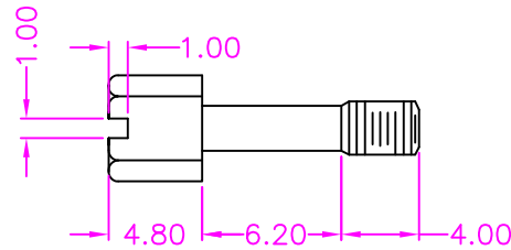
UNC #4-40 HEXSCREW
