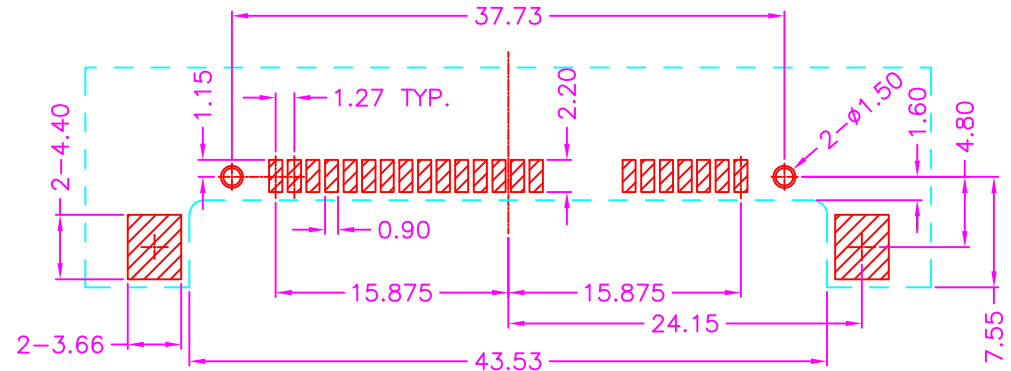
P.C.B. LAYOUT TOP VIEW ±0.05
