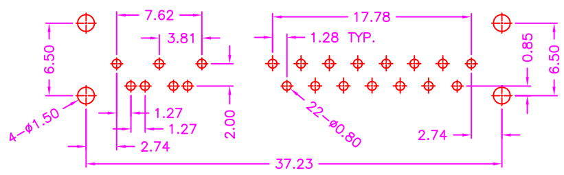
P.C.B. LAYOUT TOP VIEW ±0.05
