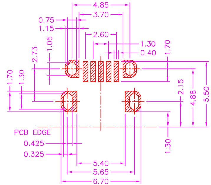
P.C.B LAYOUT TOP VIEW ±0.05
