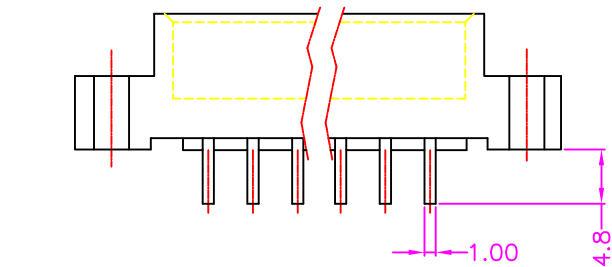
DIP TYPE
