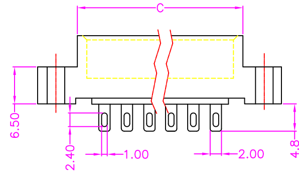
SOLDER TYPE
