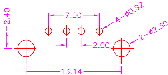
P.C.B. LAYOUT TOP VIEW ±0.05
