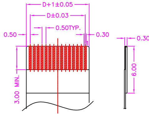
APPLICABLE FPC RECOMMENDED DIMENSION
