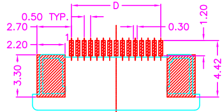
P.C.B LAYOUT TOP VIEW ±0.05
