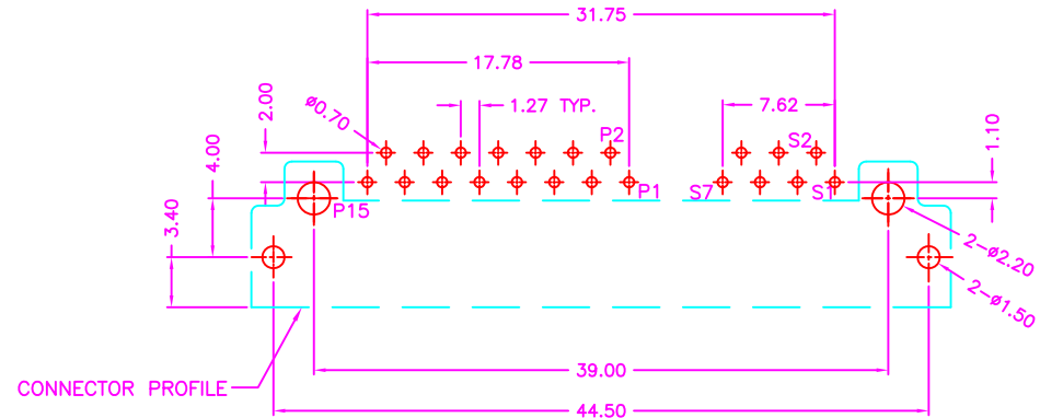
P.C.B. LAYOUT TOP VIEW ±0.05
