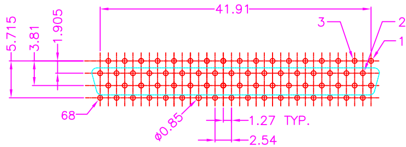
P.C.B. LAYOUT TOP VIEW ±0.05
