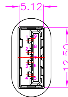
USB 3.0 FEMALE
