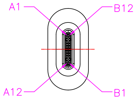
USB TYPE C MALE
