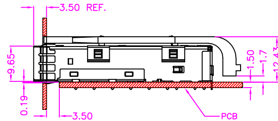
BEZEL OPENING BELOW TOP OF PCB
