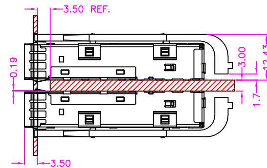
BEZEL OPENING BELOW TOP OF PCB
