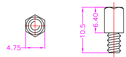
4#-40UNC SCREW
